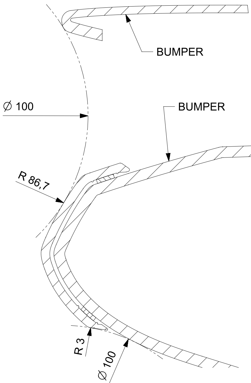
SECTION F-F
