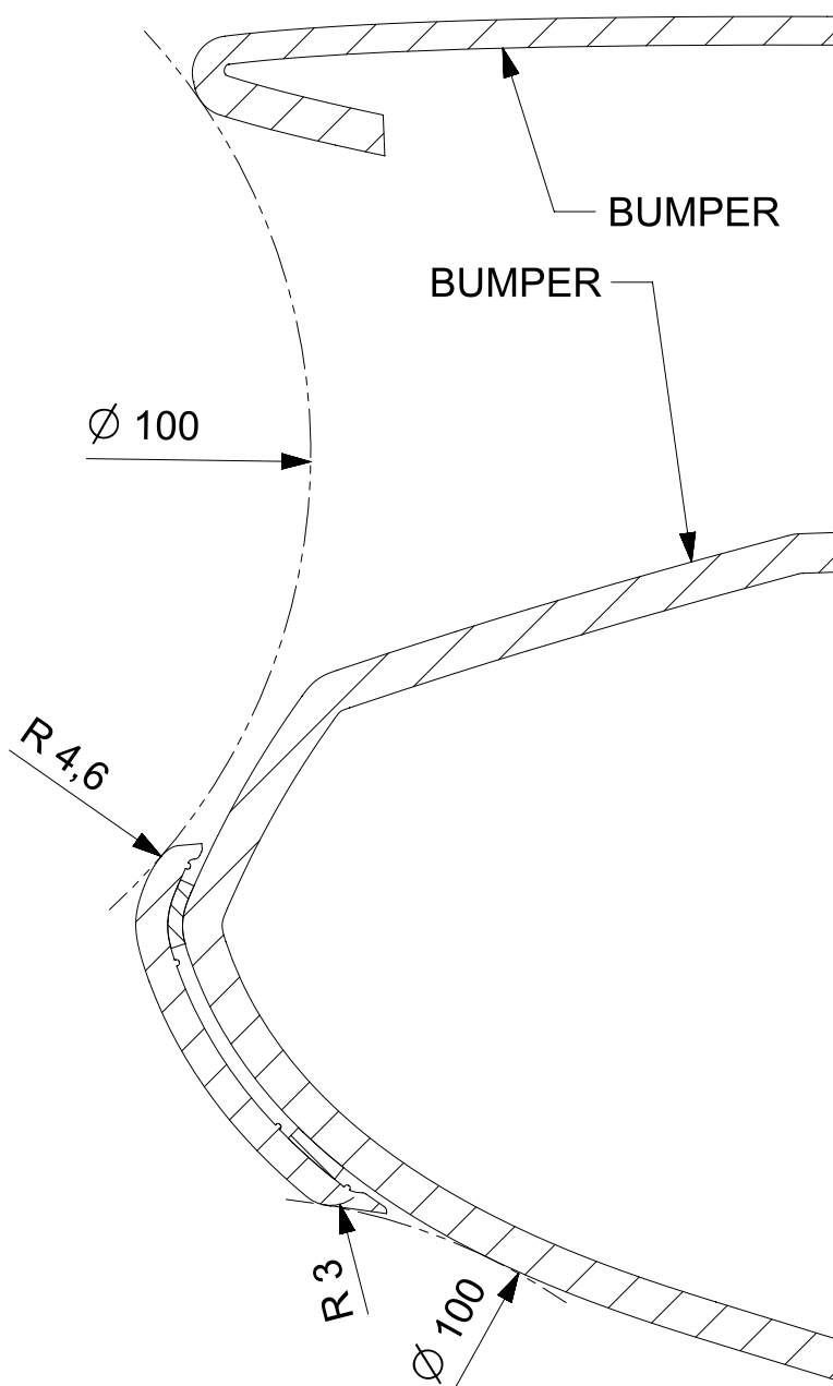
SECTION G-G
