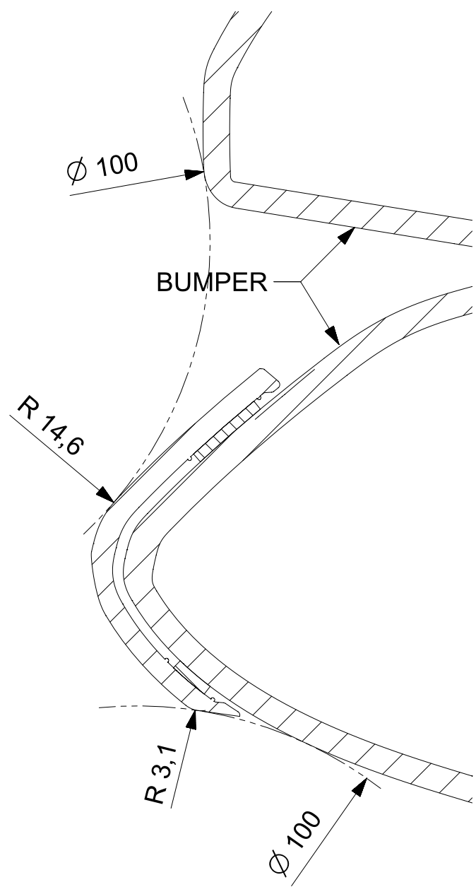
SECTION E-E
