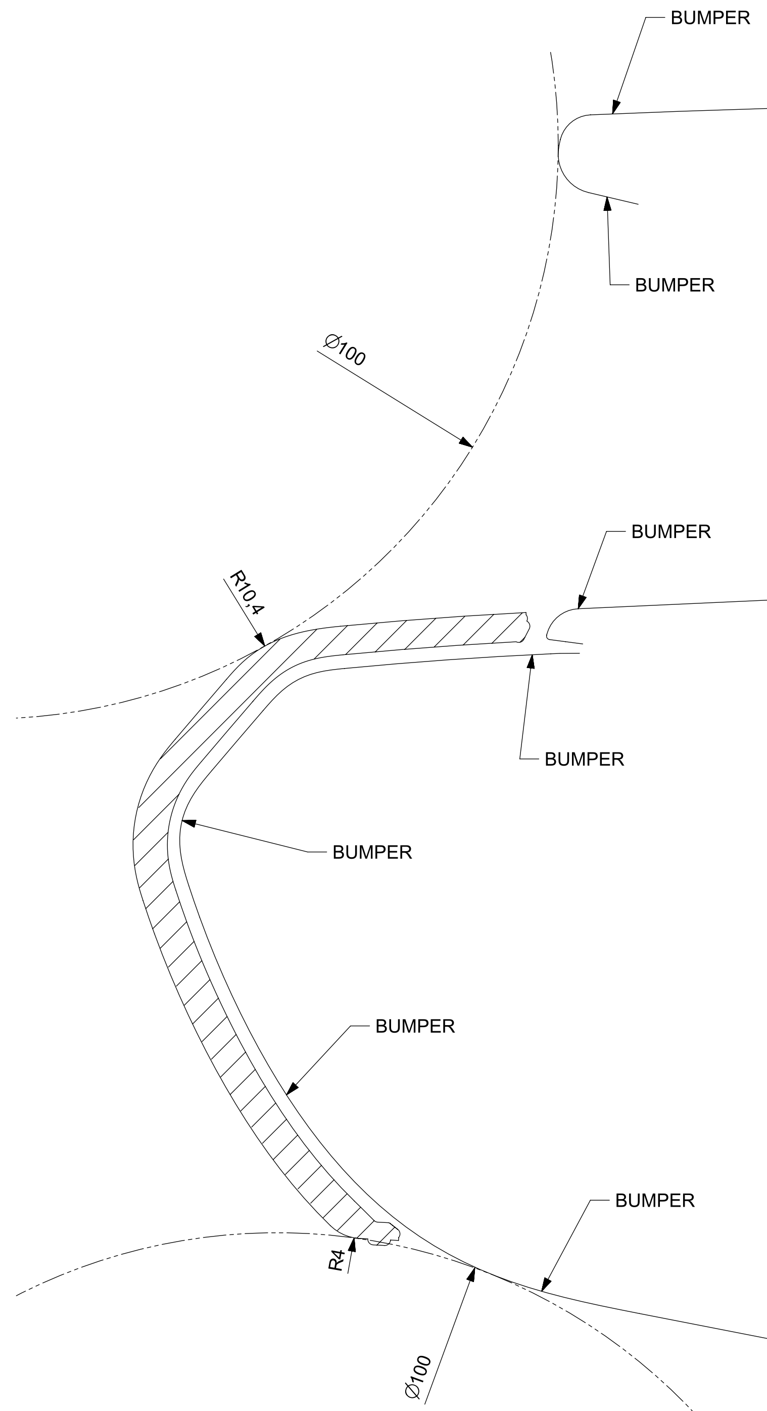
SECTION G-G
