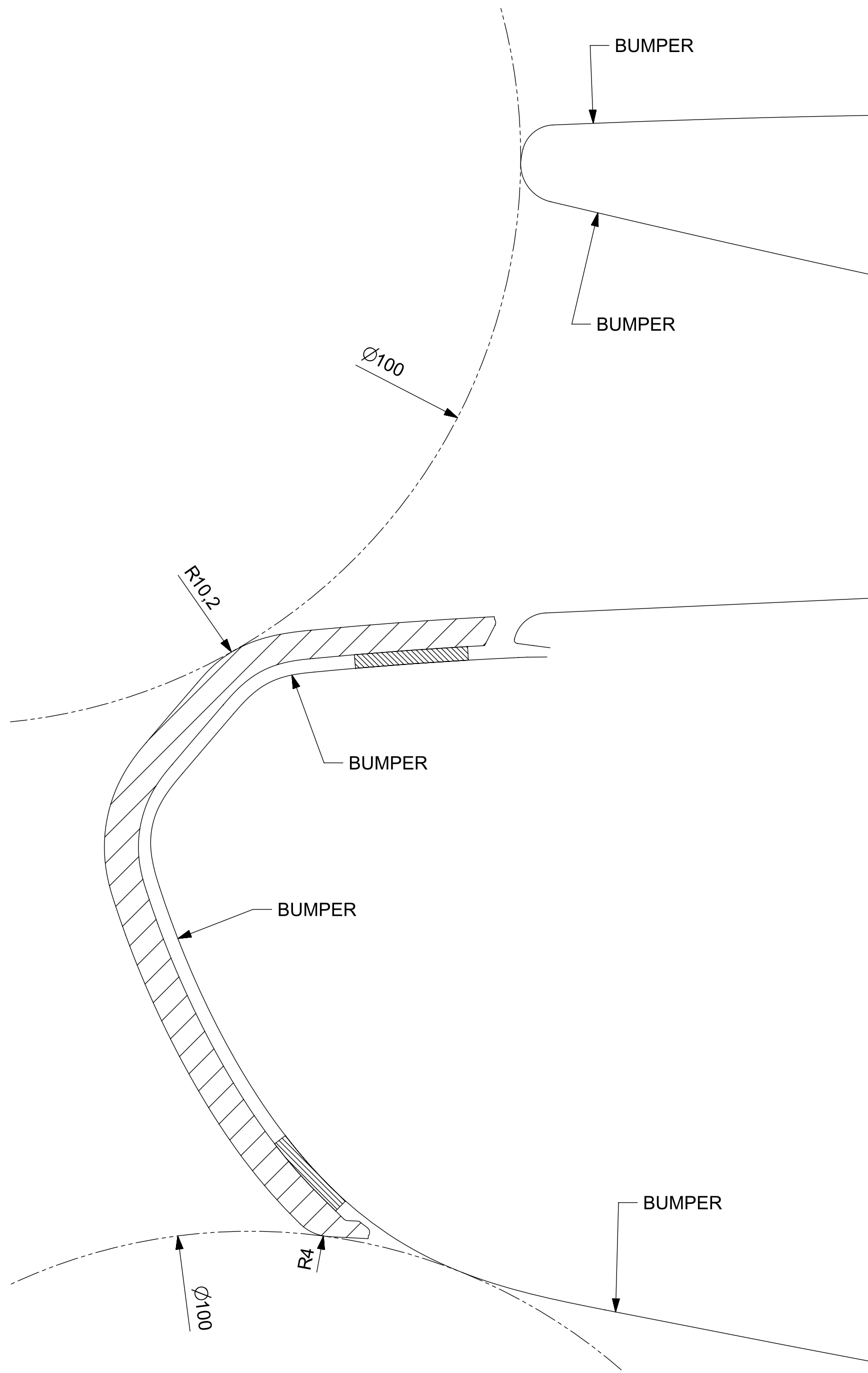
SECTION H-H
