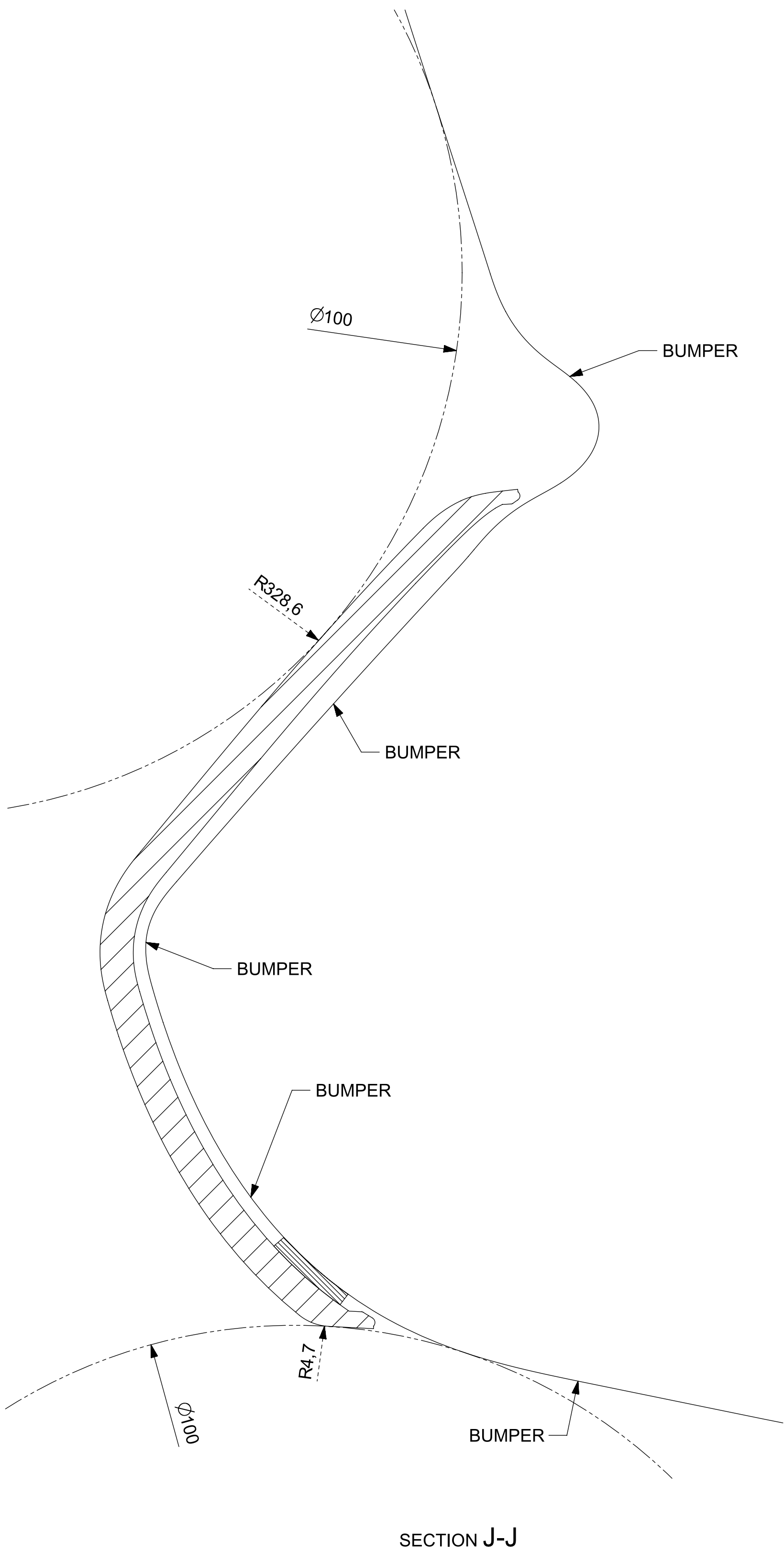
SECTION J-J
