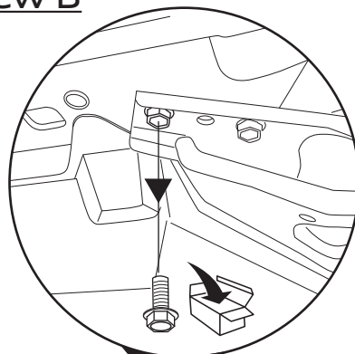
Fig.2 View B
